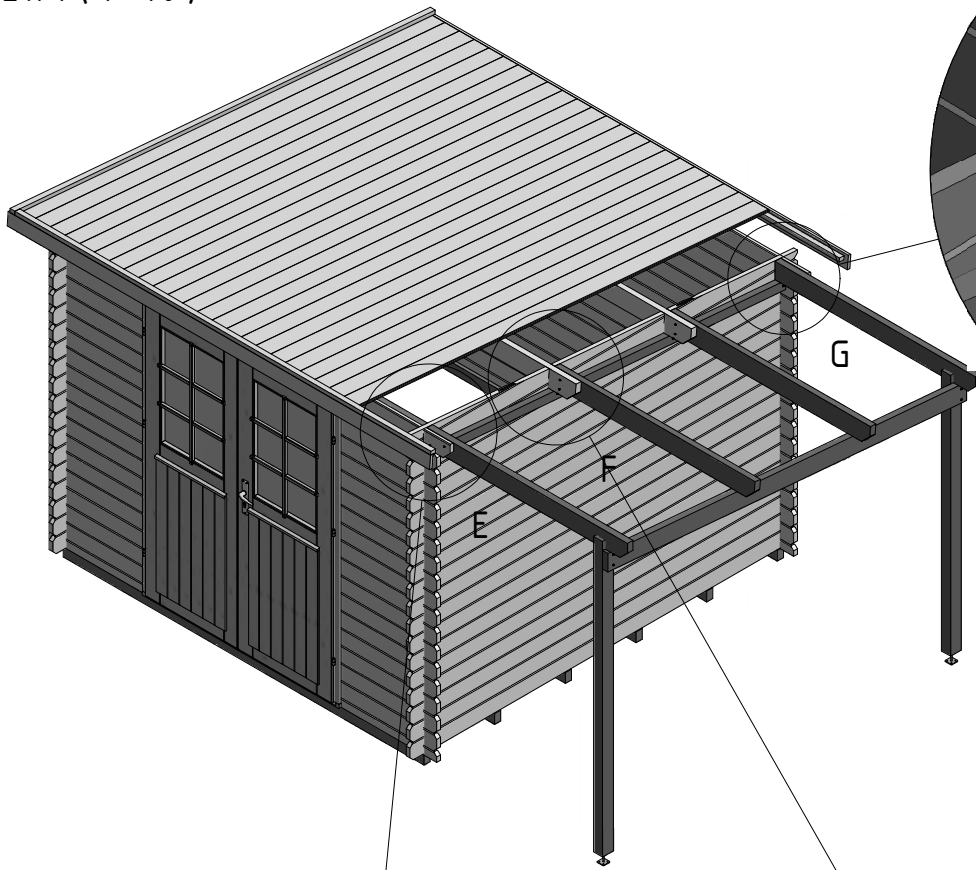
VIEW4 ( 1 : 40 )
