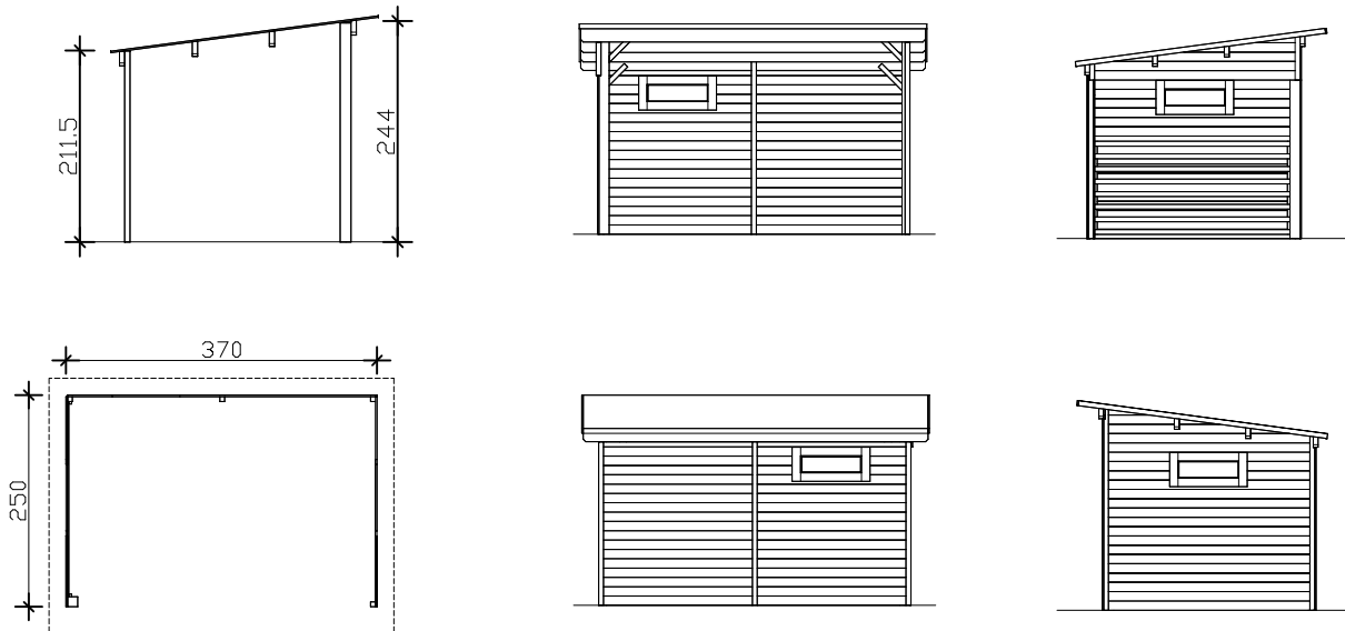
Floor plan, cross-section and elevations M 1:100
