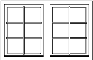
Dobbeltvindue / Double window 4 st. 70 mm 1530 x 990 mm
